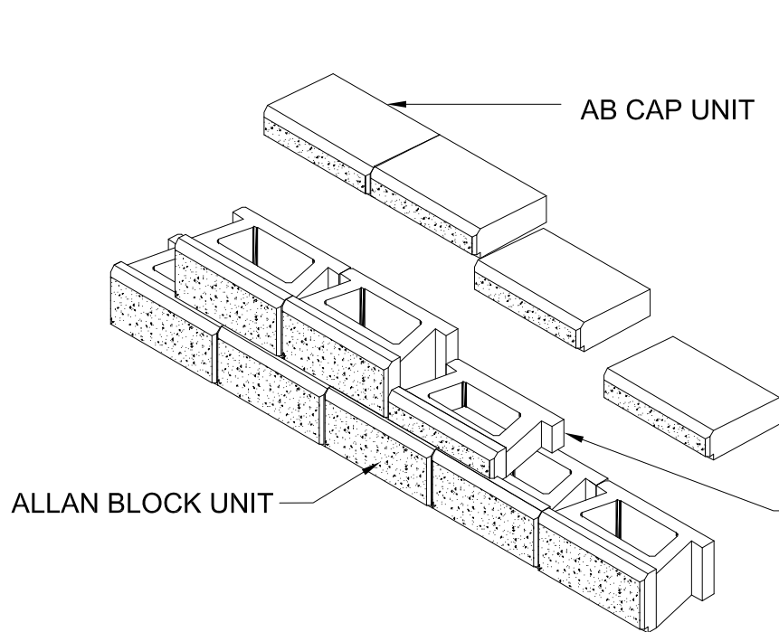
AB TYPICAL SECTION – STEP UPS WITH AB LITE STONE
