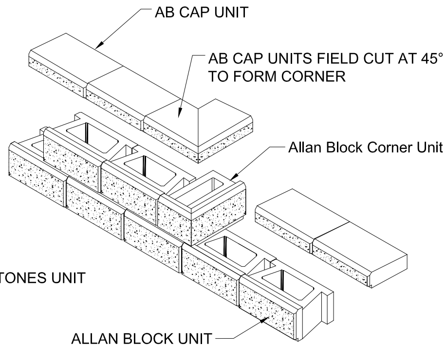
AB TYPICAL SECTION – FULL COURSE STEP UPS WITH AB CORNER BLOCK
